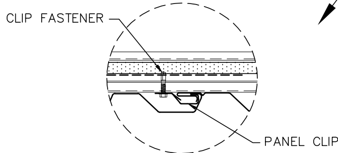
PANEL CLIP
